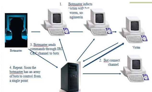
Fig1: Botnet Mechanism
