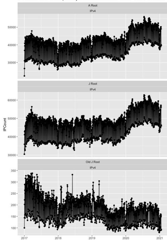
Number of Distinct IPs per Day at A and J Root Servers for .CORP Queries
