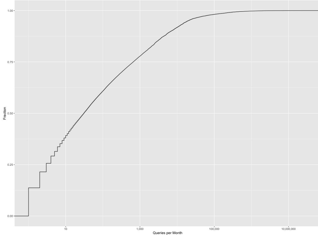
CDF of Number of Queries Sent by IP for .CORP
