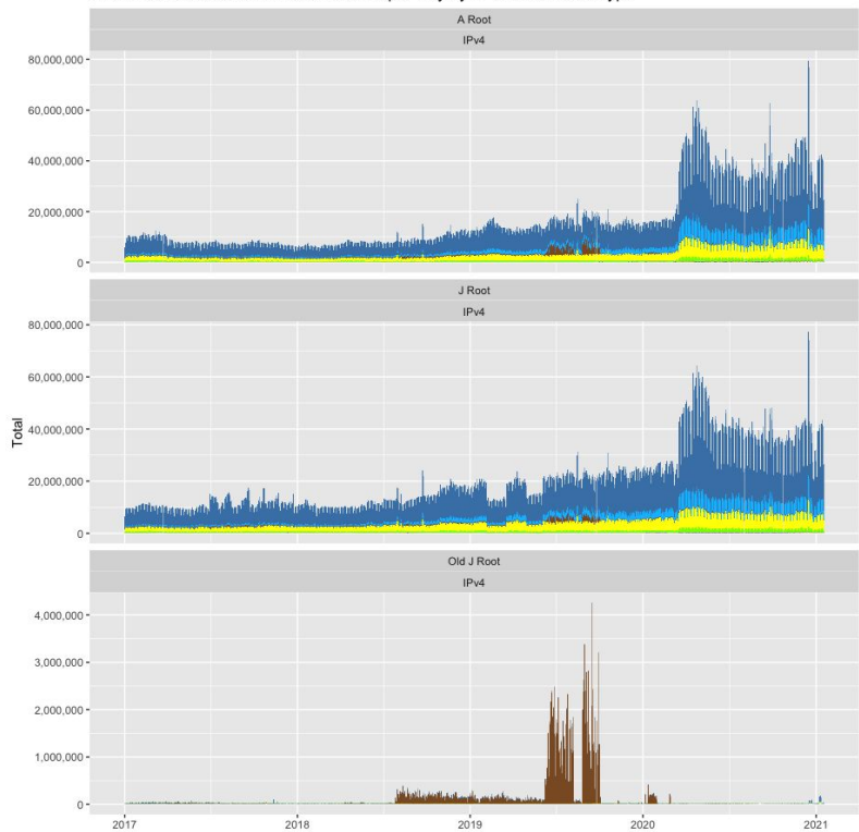
.CORP Queries to A and J Root Servers per Day by IP Version and QType
