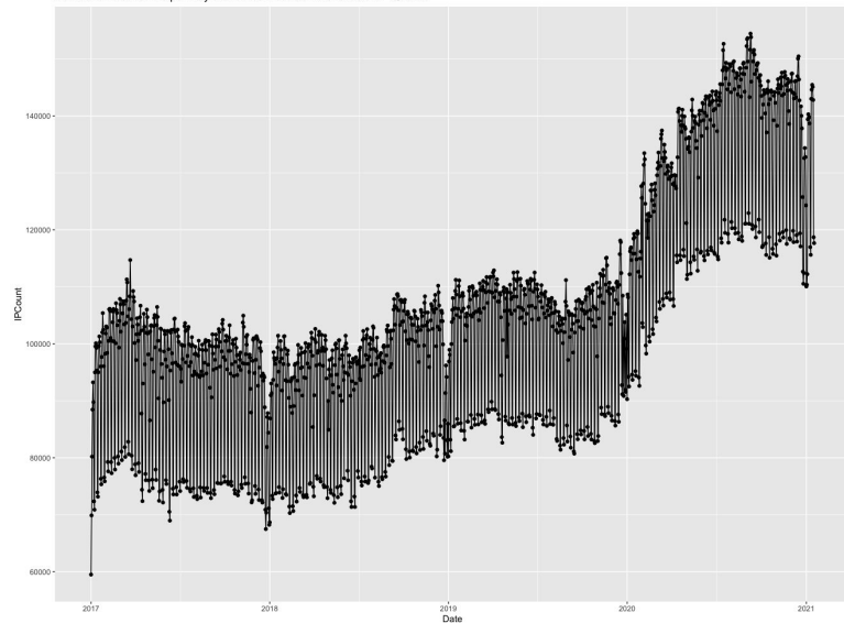
Number of Distinct IPs per Day at A and J Root Servers for .CORP Queries
