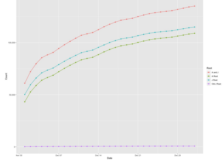
Cummulative Unique IP Addresses Querying .CORP (Minimum 10 Queries)
