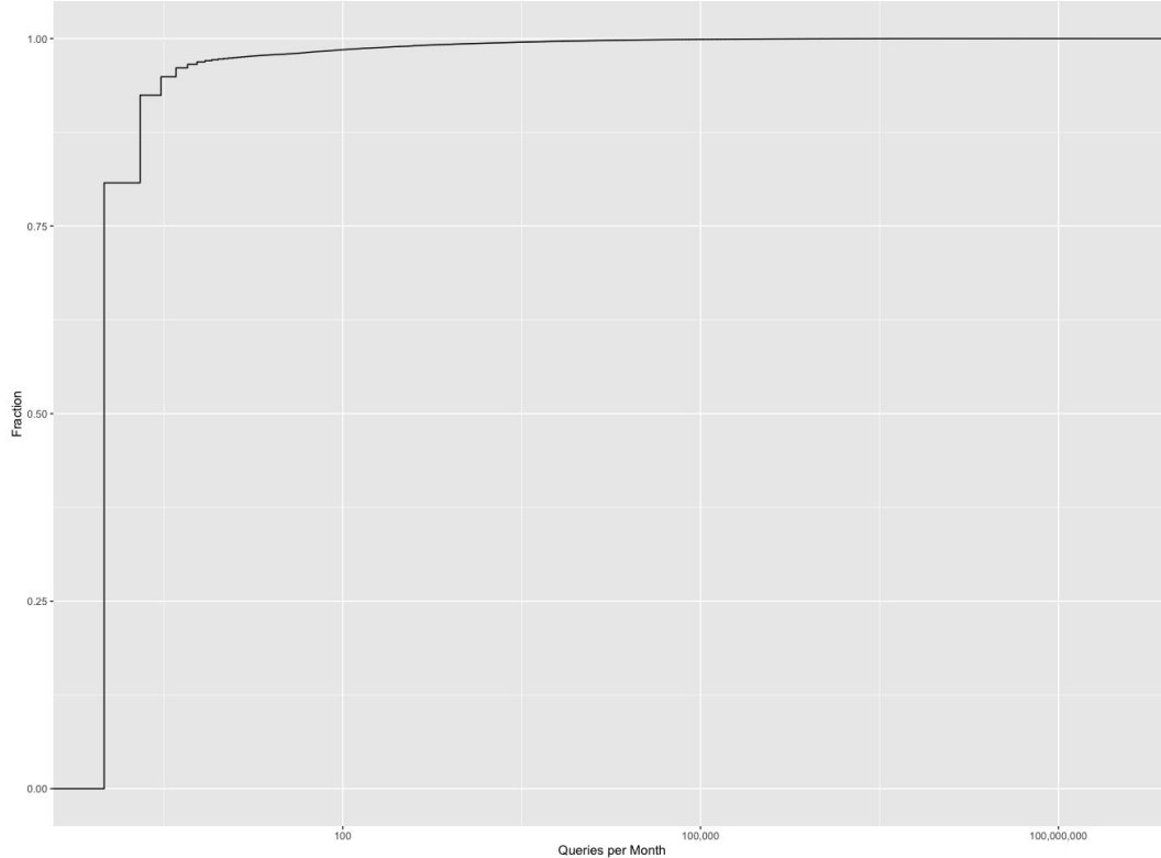
CDF of Number of Queries per SLD for .CORP
