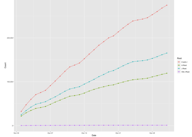
Cummulative Unique SLDs for .CORP (Minimum 2 Queries)
