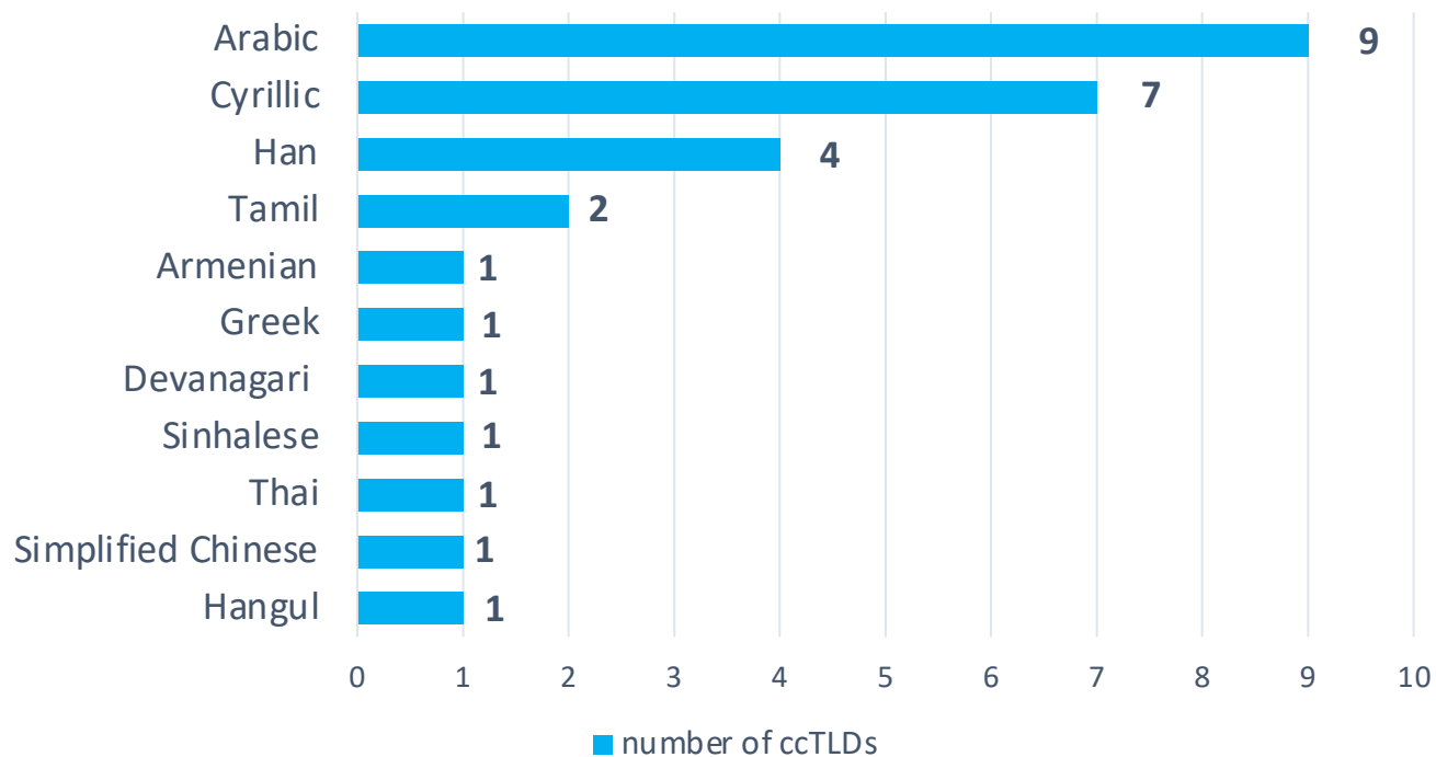
Scripts offered in IDN ccTLDs surveyed
